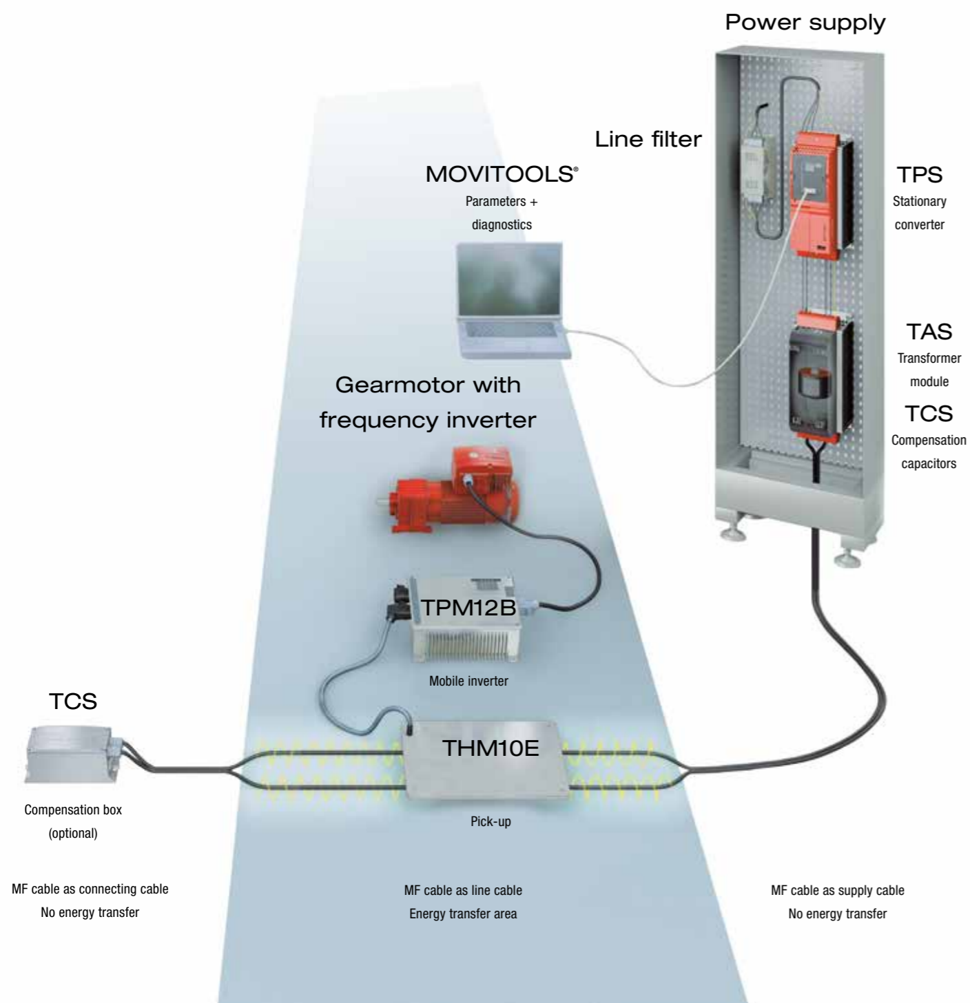
MOVITRANS® with flat pick-up (THM10E)
